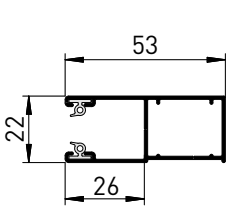
HTF-DRP (511)
