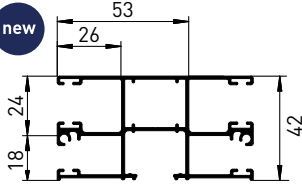
M-F-HTF-IS DRP (5045)
