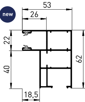
F-HTF-K 40-DRP (514)
