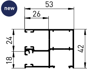
F-HTF-IS DRP (5044)
