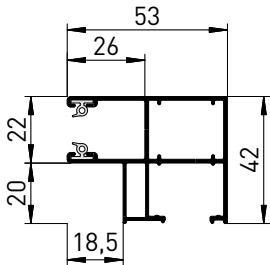
F-HTF-K 20-DRP (512)
